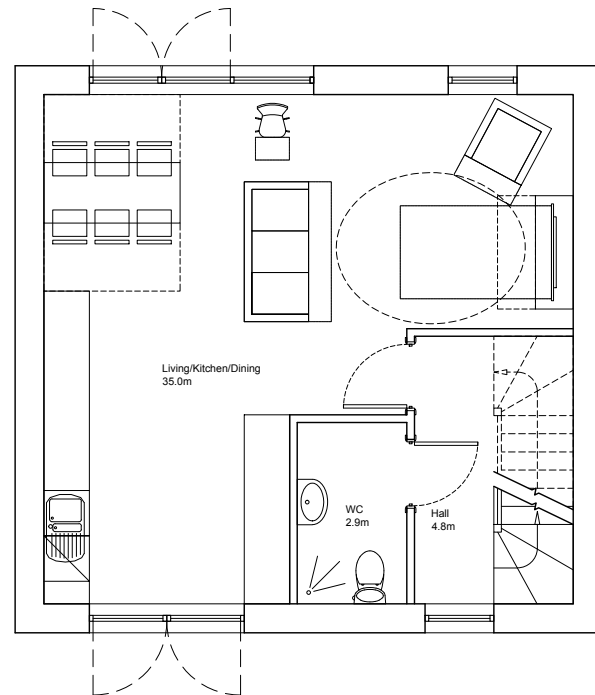
HOUSE TYPE A (TERRACED) GROUND FLOOR PLAN GROSS INTERNAL AREA- 47.1 m 2
