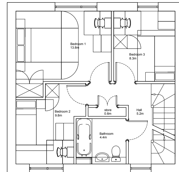
HOUSE TYPE A (TERRACED) FIRST FLOOR PLAN GROSS INTERNAL AREA- 47.1 m 2
