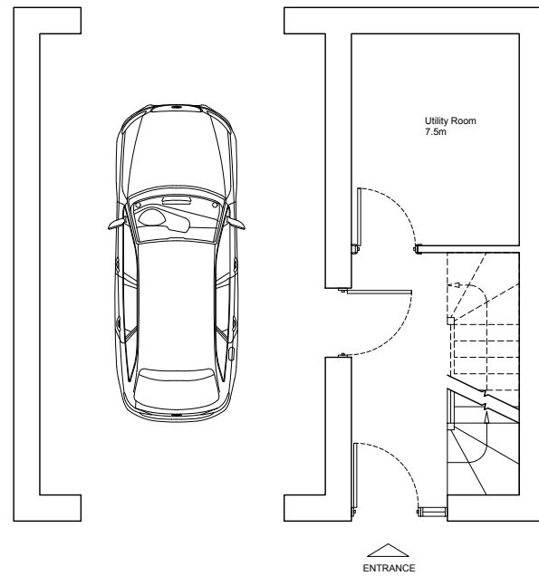
HOUSE TYPE A (TERRACED) - 4Bed/6persons TOTAL GIA - 142.6 m 2 LOWER GROUND FLOOR PLAN GROSS INTERNAL AREA- 16.5 m 2
