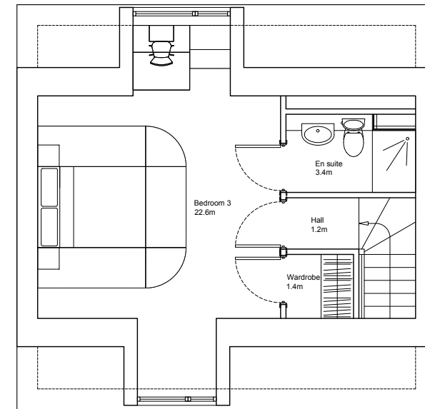
HOUSE TYPE A (TERRACED) SECOND FLOOR PLAN GROSS INTERNAL AREA- 31.9 m 2
