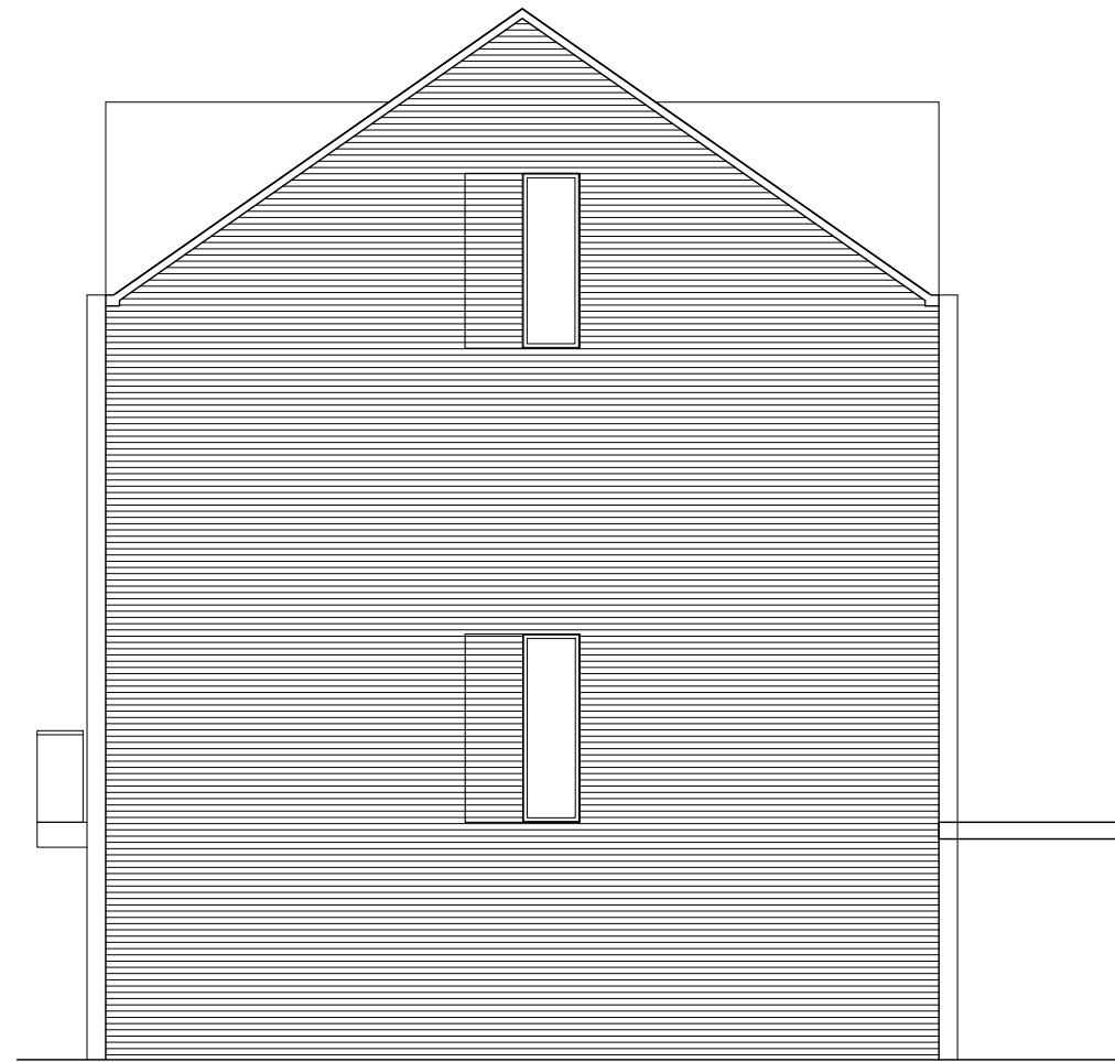
Side Elevation (East)
