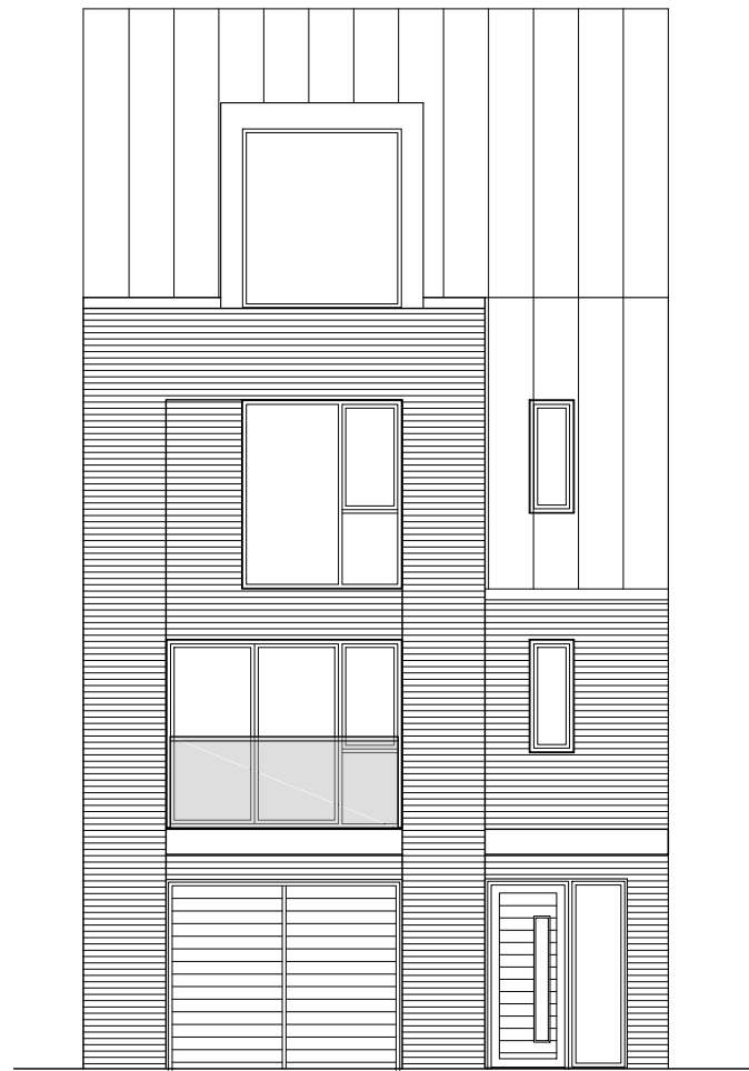
Front Elevation (South)
