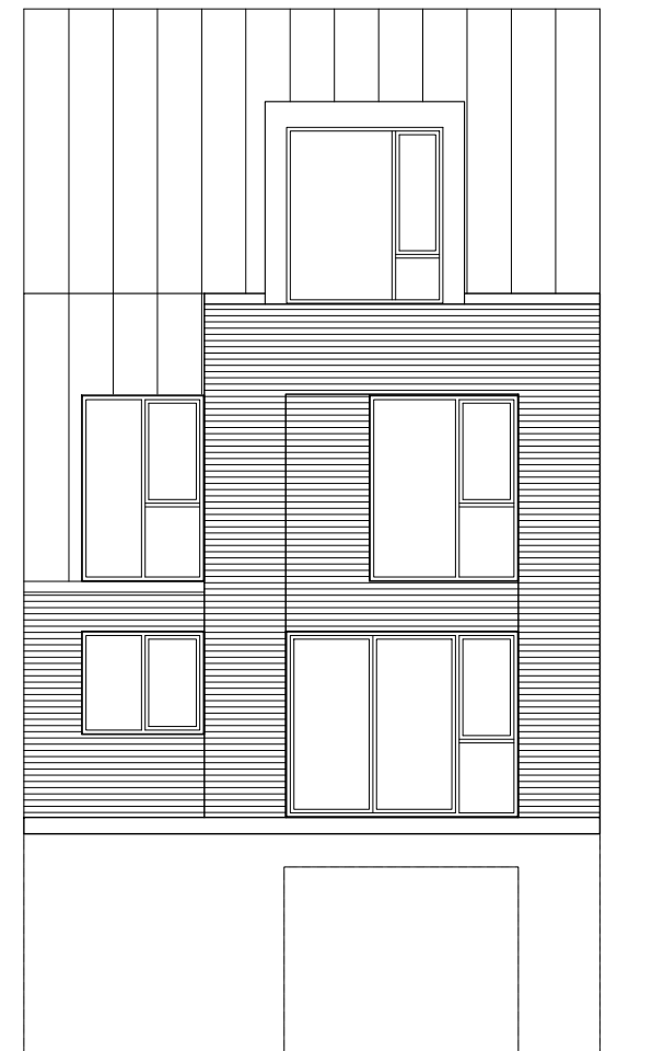
Back Elevation (North)
