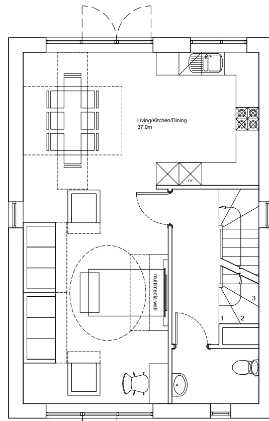
HOUSE TYPE B (DETACHED) GROUND FLOOR PLAN GROSS INTERNAL AREA- 57.2 m 2
