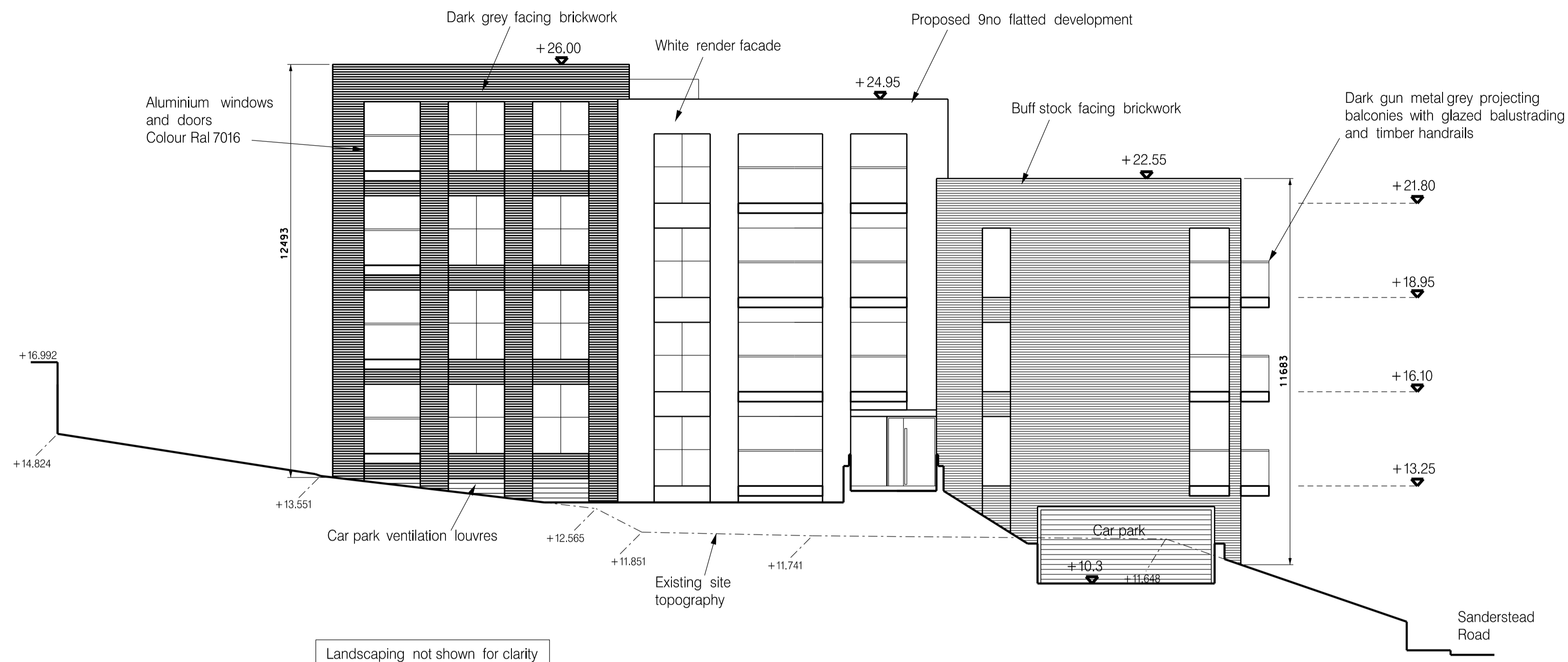
PROPOSED NORTH WEST ELEVATION (WEST HILL)
